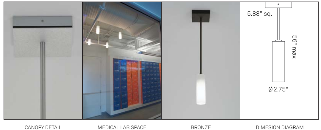
CANOPY DETAIL
